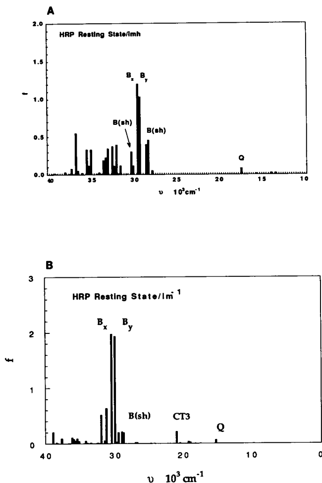
FIGURE 2 Calculated absorption spectra of HRP resting state with (A) an imidazole ligand, and (B) an imidazolate ligand.
