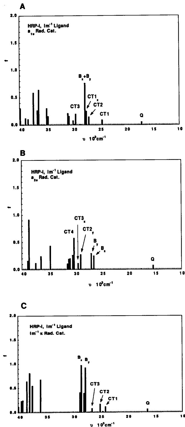
FIGURE 4 Calculated absorption spectra of HRP-I with the \text{im}^{-1} ligand (A) in the a_{1u} radical cation state, (B) in the a_{2u} radical cation state, and (C) in the \text{im}^{-1} \pi_3 radical cation state.
